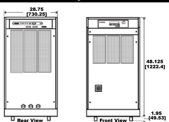
MX30/MX45 Dimensions - single chassis
