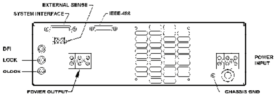
751L / 1501L / 2001L REAR PANEL
